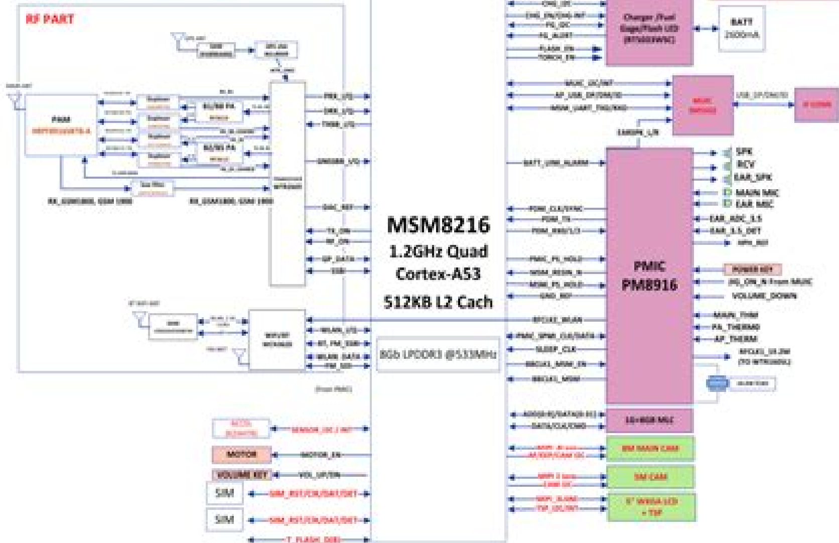
1M-GS30H/DSREV1.0 Block Diagram
