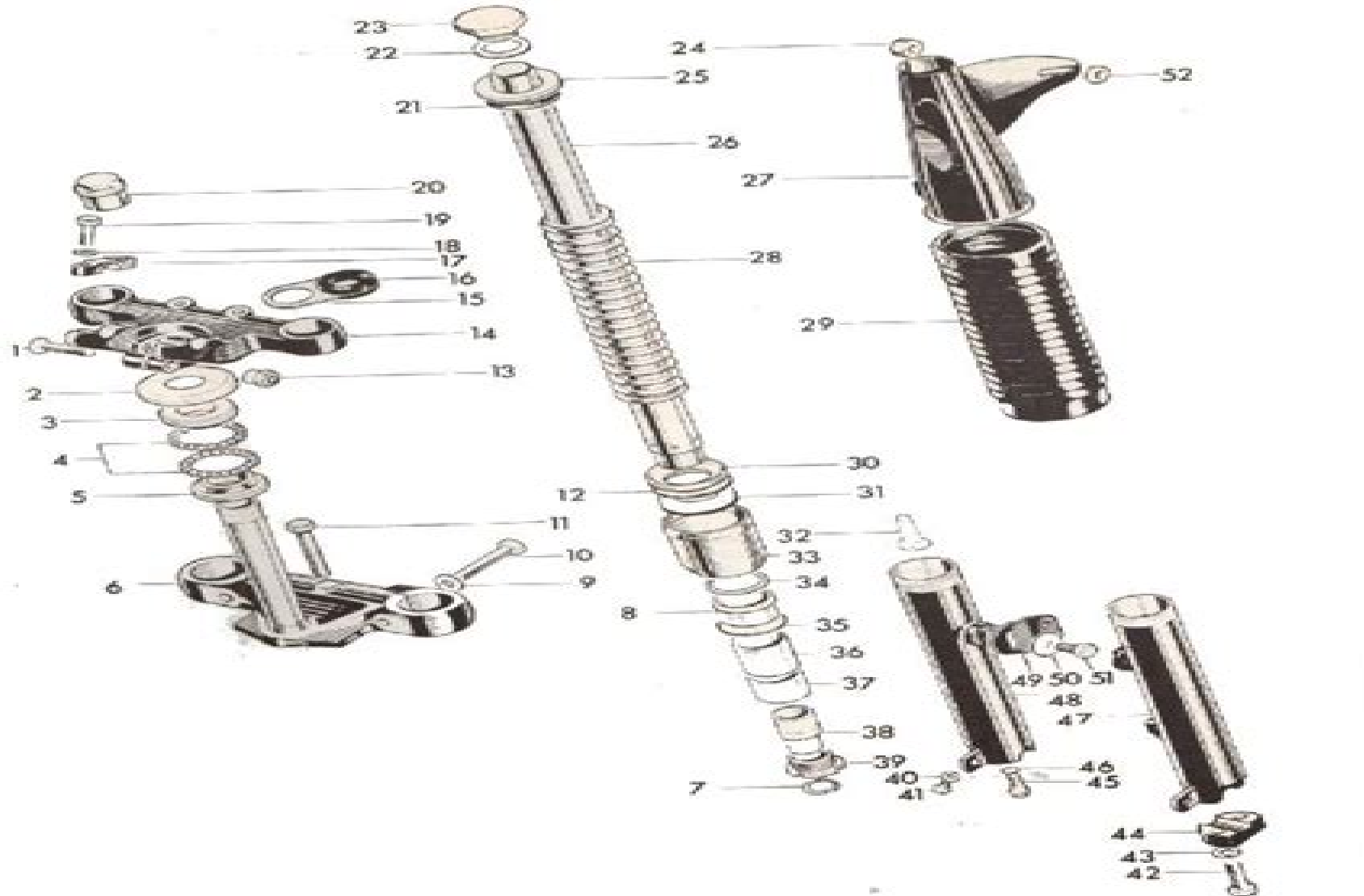
EXPLODED VIEW OF THE SHUTTLE TYPE FRONT FORKS FITTED TO MACHINES PRIOR TO 1970
