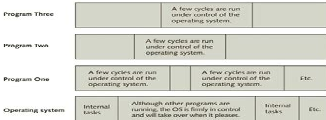
Figure 1-10 Preemptive multitasking basics
