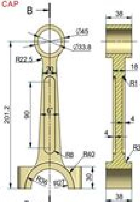
SECTION B-B 04. CONNECTING ROD
