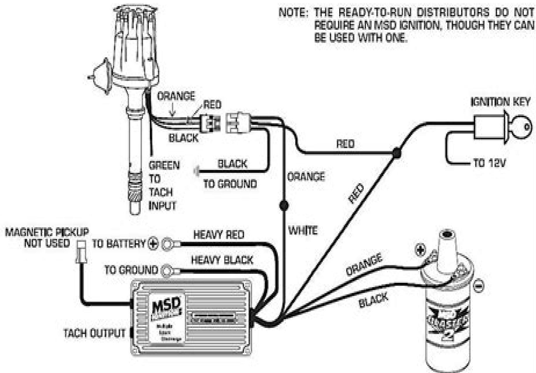
Figure 11 Connecting an MSD Ignition Control to the Ready-to-Run Distributor.
