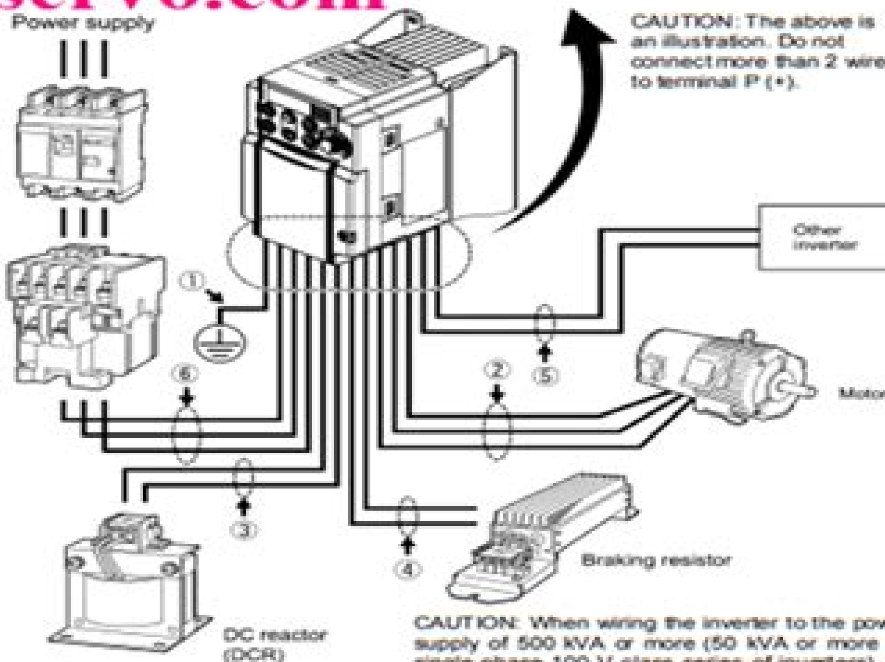
Figure 2.4 Wiring Procedure for Peripheral Equipment
